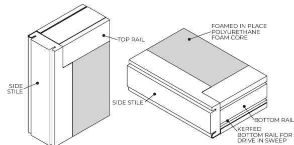
STILE & RAIL CONSTRUCTION DETAIL
